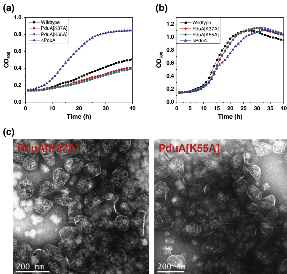
Fig. 8. PduA-K37A and PduA-K55A phenotype. Respective strains were grown on minimal 1,2-PD medium with (a) limiting (20 nM) or (b) saturating (100 nM) CN-B 12 , respectively. The growth curves were repeated at least three times in duplicate and representative curves are shown. (c) Electron micrographs of purified PduA-K37A and PduA-K55A MCPs.
