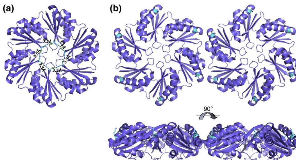
Fig. 11. Structural positions of K37 and K55 in PduA. (a) Six PduA K37 residues form a ring-like structure stabilized by hydrogen bonds. This ring may be important for the function of the central pore, which is thought to act as a conduit for 1,2-PD. (b) K55 is located near the vertices of PduA hexamers.
