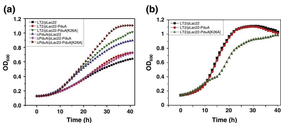
Fig. 4. PduA-K26A dominance test. Production of PduA-K26A from a plasmid in an otherwise wild-type strain resulted in phenotypes indicative of a broken MCP: fast growth at limiting B_{12} (a) and temporary growth inhibition at saturating B_{12} (b). This indicated that the PduA-K26A phenotype was dominant. Respective strains were grown on minimal 1,2-PD medium with (a) limiting (20 nM) or (b) saturating (100 nM) CN-B_{12} , respectively. The growth curves were repeated at least three times in duplicate and representative curves are shown.
