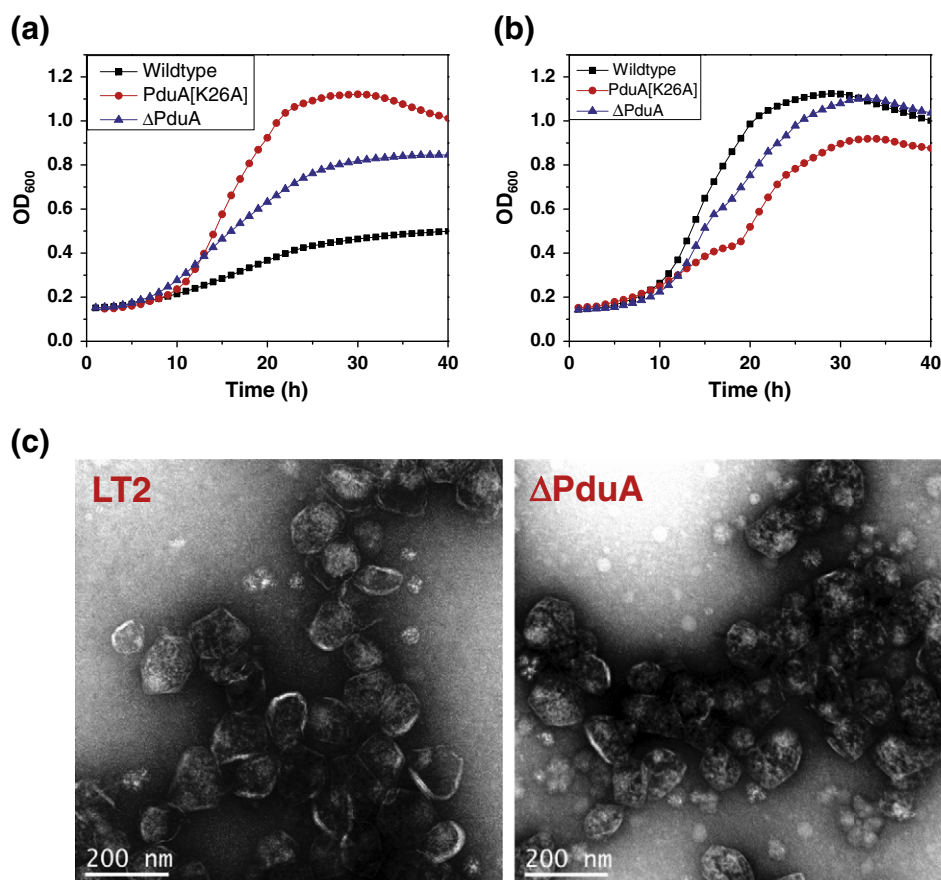
Fig. 3. PduA-K26A phenotype. Respective strains were grown on minimal 1,2-PD medium with (a) limiting (20 nM) or (b) saturating (100 nM) CN-B 12 , respectively. The growth curves were repeated at least three times in duplicate and representative curves are shown. (c) Electron micrographs of purified wild type and ΔPduA MCPs. The PduA-K26A strain did not yield any MCPs.
