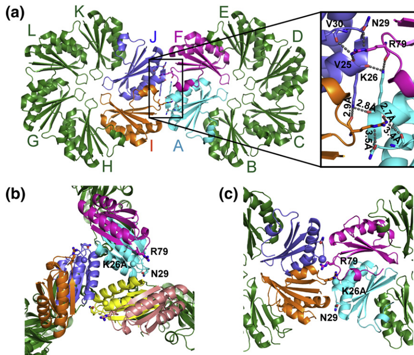
Fig. 10. PduA inter-hexamer interactions. (a) The interface is stabilized by 10 sets of interactions contributed by four different monomers. As indicated in the figure, interacting subunits A (cyan) and F (magenta) are from one hexamer and interacting subunits I (orange) and J (light blue) are from another hexamer. The important interactions are listed in Table 4. (b) PduA-K26A crystal structures contain new edge-to-face interactions not present in wild-type PduA. (c) Crystal form 1 of PduA-K26A also has drastically altered edge-to-edge interactions between hexamers. The \beta -carbon of the alanine mutation is highlighted as a sphere in (b) and (c).
