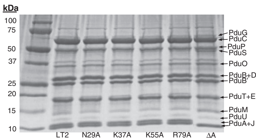
Fig. 7. SDS-PAGE gel of purified MCPs. Ten micrograms of Pdu MCPs purified from wild-type Salmonella or respective mutants was loaded onto a 10–20% SDS-PAGE gel. The respective lanes of the mutants are indicated on the gel.
